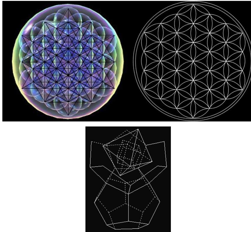
Platonic solids in the nucleus of the atom
