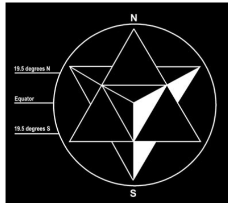
Star Tetrahedron
