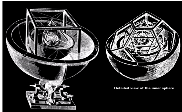
Kepler Model
