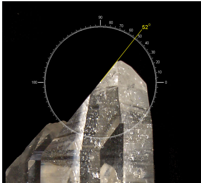
Quartz Crystal
