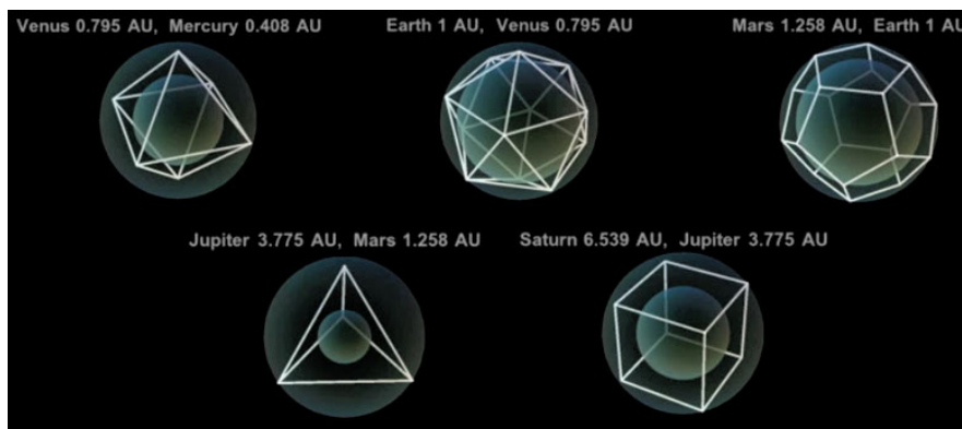
Planetary Orbits
