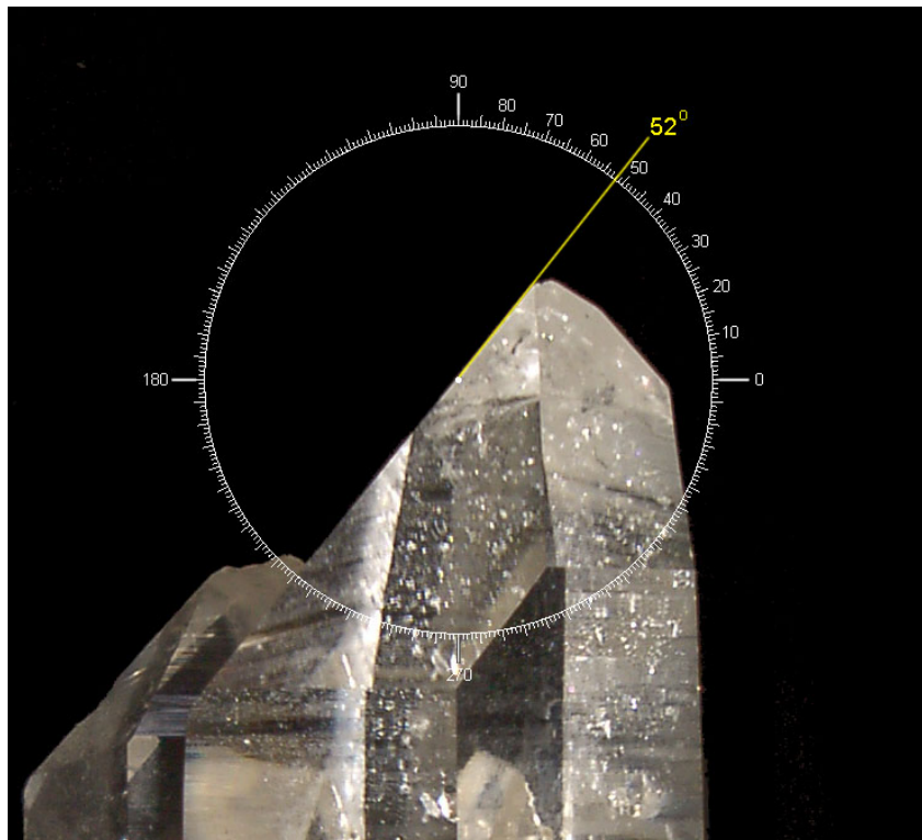
Quartz Crystal
