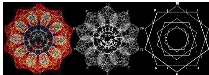
DNA dodecahedron model showing the 20 standard amino acids organized in space according to water affinity.
