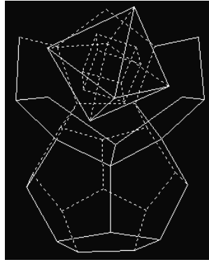
Platonic solids in the nucleus of the atom
