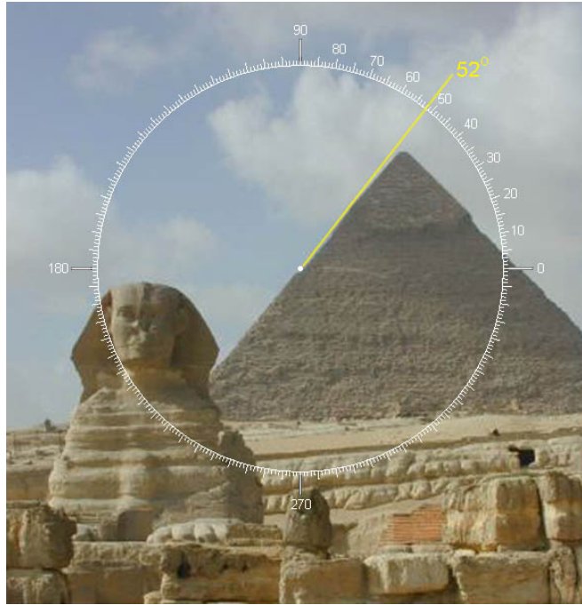
52 degree angle of the Great Pyramid
