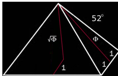
52 degree (51.843) angle of the Great Pyramid and the relationship to Phi
