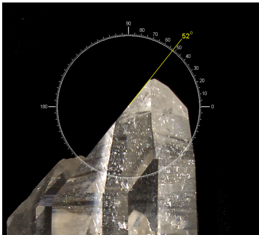
52 degree angle of quartz crystal
