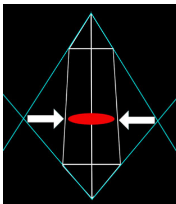
The red disc is the area of the vortex
